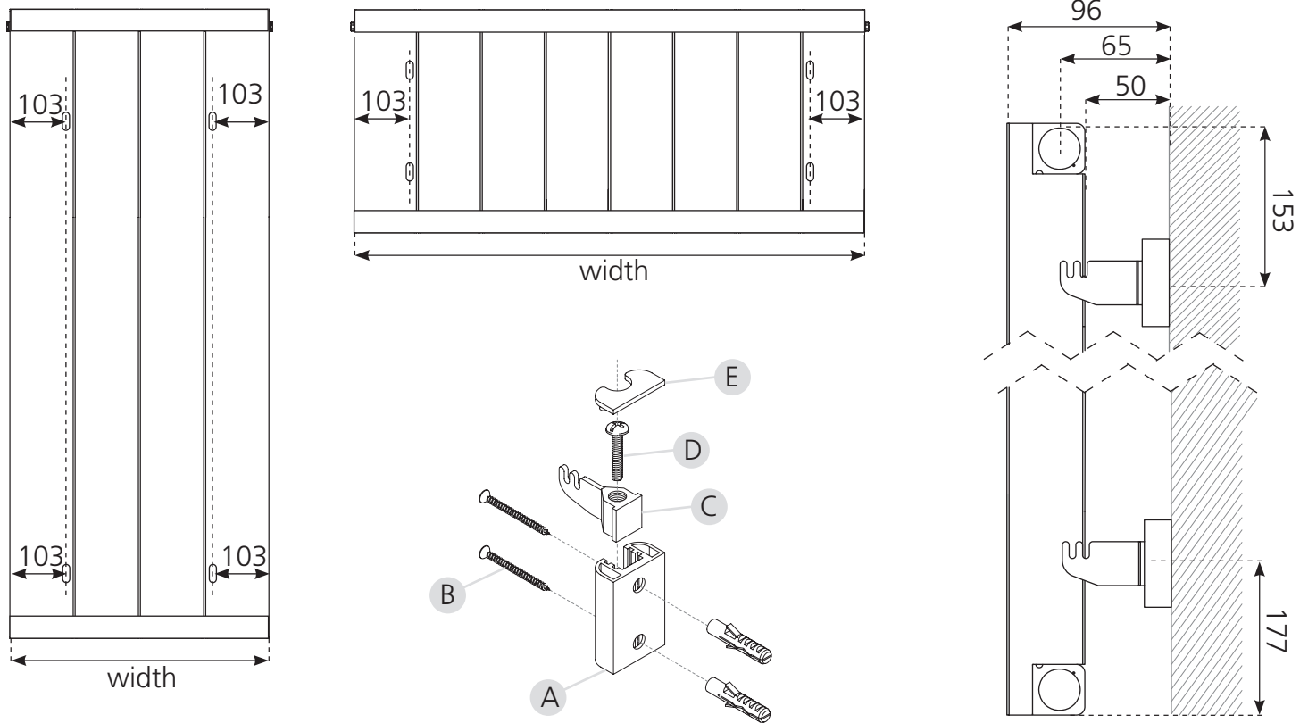
Drawing 1 - Fixing Positions for Brackets
