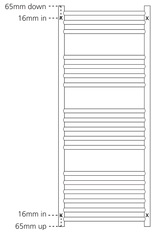
Drawing 3 - Bracket Positions
