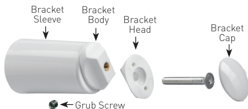
Fig 2. Bracket Assembly
